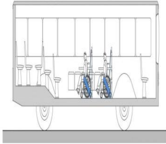
Bus layout for group travel with four wheelchair positions, two on each side
