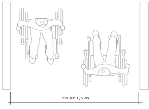
Image 93. Min net width for 2 wheelchairs passage
